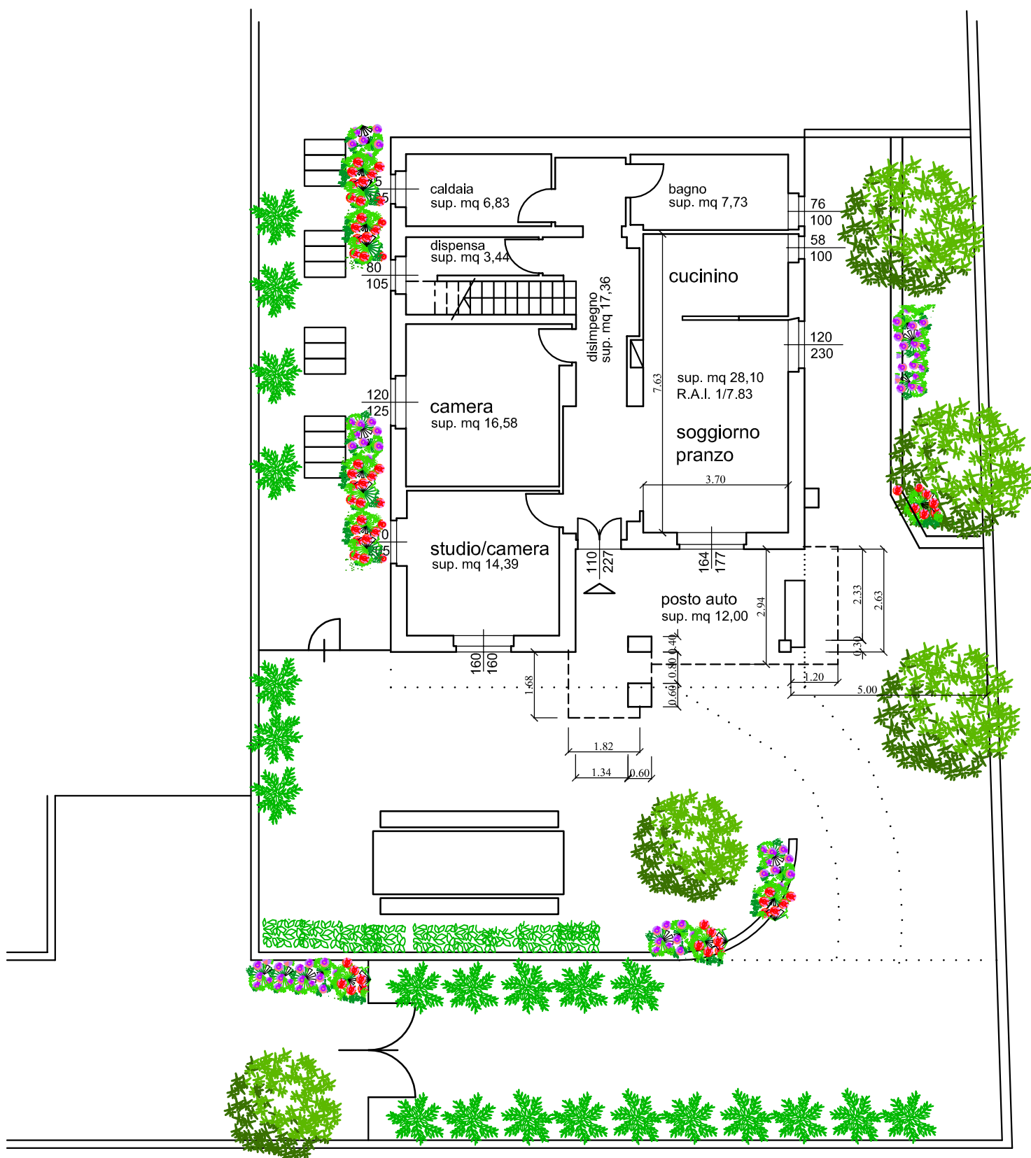
PIANO TERRA
